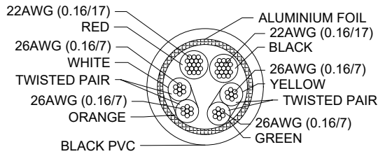
CABLE BUILDUP
