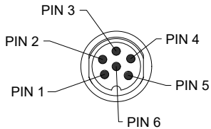
6 PIN MALE CONNECTOR
