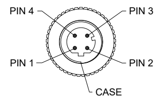
4 PIN M12 MALE D-CODED CONNECTOR
